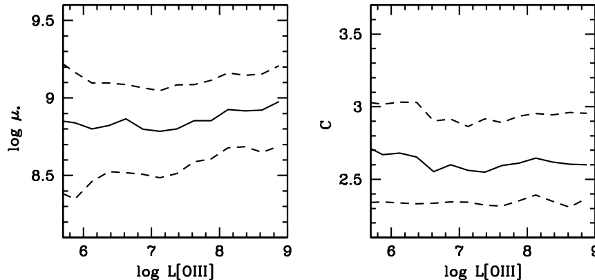
Figure 8: The stellar surface density \mu_* and concentration index C are plotted as functions of \log L[\text{OIII}] for the AGN in our sample. The solid line shows the median, while the dashed lines indicate the 16-84 percentiles of the 1/V_{max} weighted distribution.
